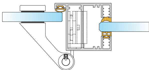
All-glass | door frame P10 | Just 3D | up to 32 dB
