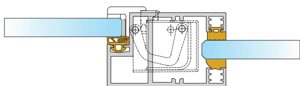
All-glass | door frame P09 | Tectus TEG 310 | up to 32 dB
