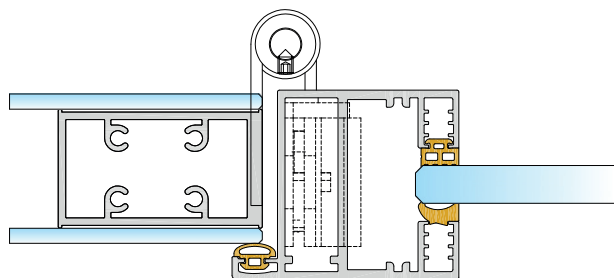
GlassDesign | door frame P10 | Just 3D | up to 34 dB
