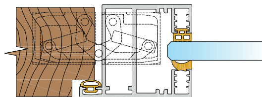
Wooden | door frame P10 | Tectus TE 340 | up to 37 dB
