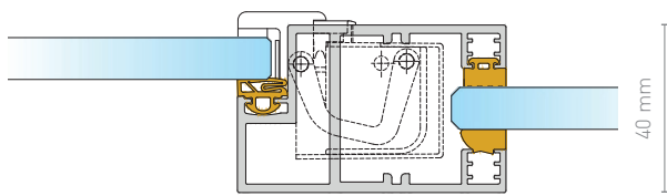
All-glass | door frame P09 | Tectus TEG 310 | up to 32 dB
