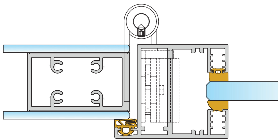
GlassDesign | door frame P10 | Just 3D | up to 34 dB
