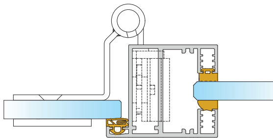
All-glass | door frame P10 | Just 3D | up to 32 dB
