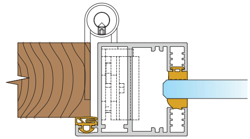
Wooden | door frame P10 | Just 3D | up to 37 dB
