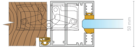
Wooden | door frame P10 | Tectus TE 340 | up to 37 dB
