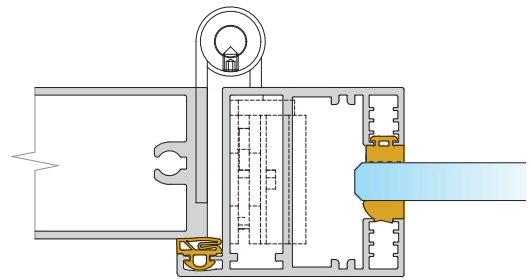
Aluminium | door frame P10 | Just 3D | up to 37 dB
